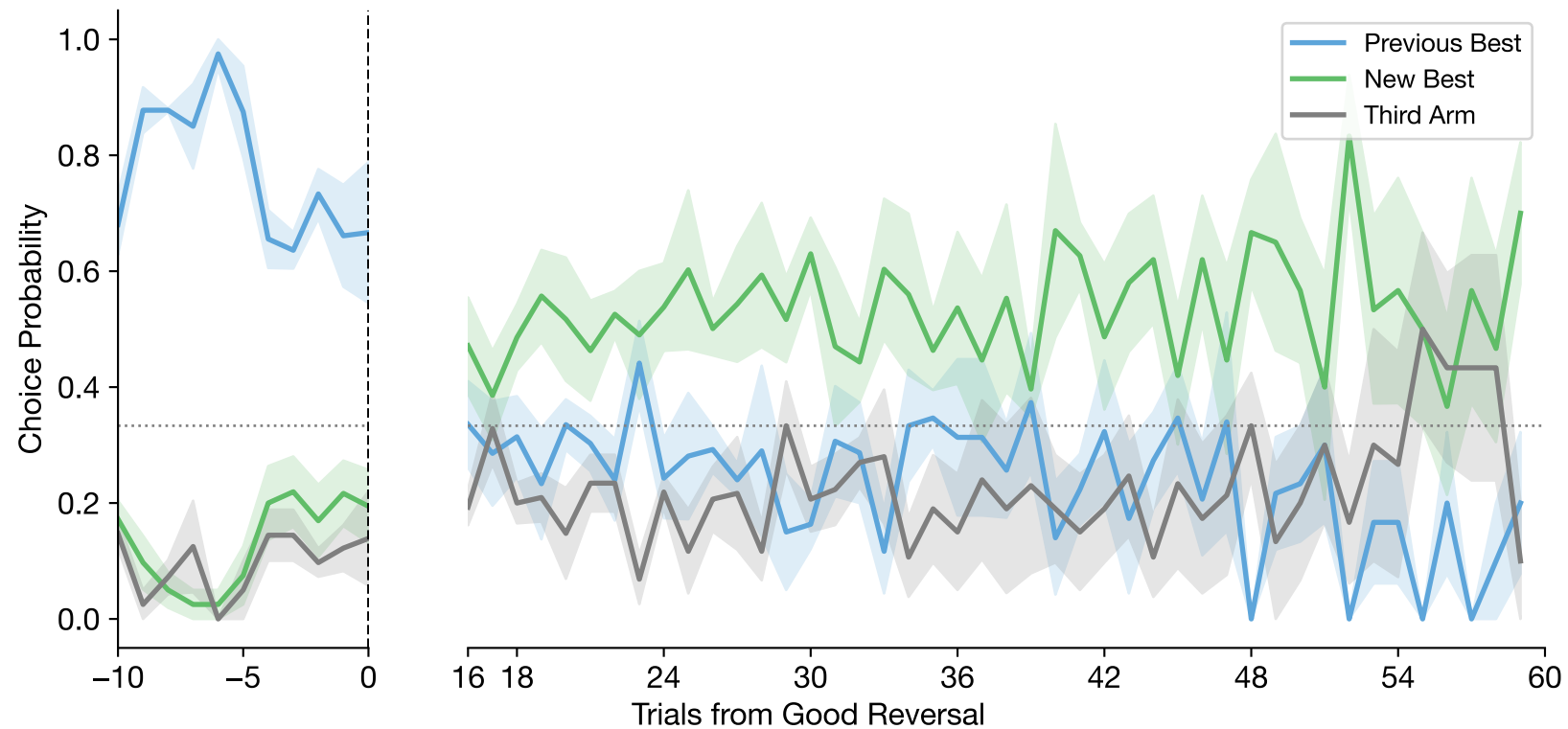
Good Reversal-Aligned Choices (mean \pm se across subjects | n=5 subjects, n=41 reversals) (Skipping first 15 trials post-reversal)
